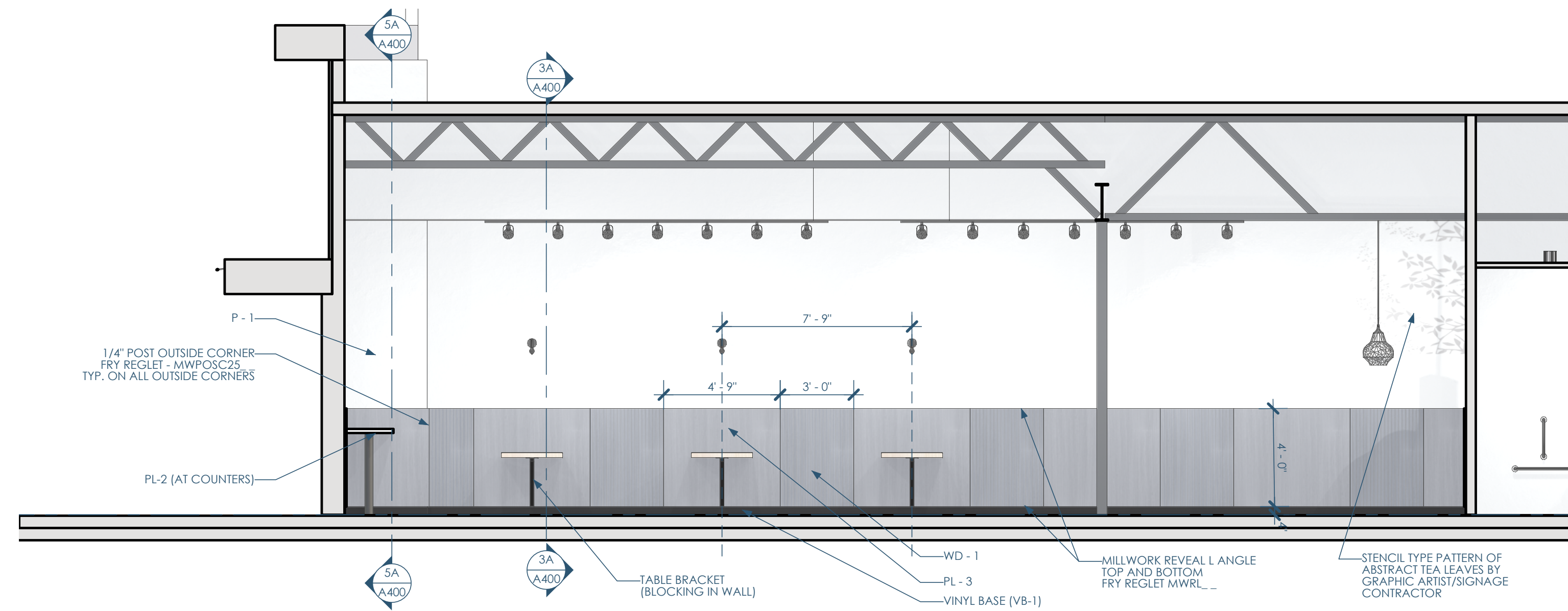
4B/A400 SECTION - SOUTH - BOOTH 1/4"=1'-0"
