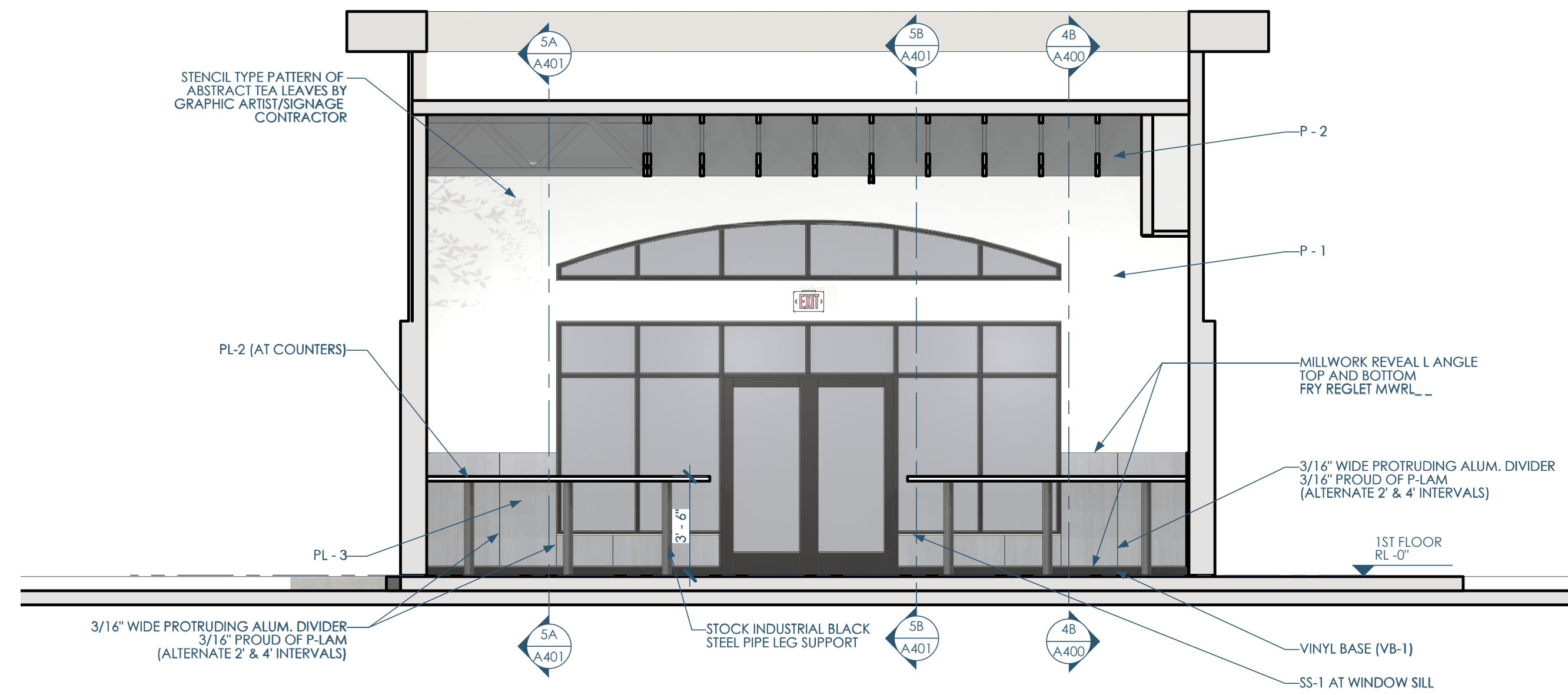
5A/A400 SECTION - EAST - FRONT 1/4"=1'-0"
