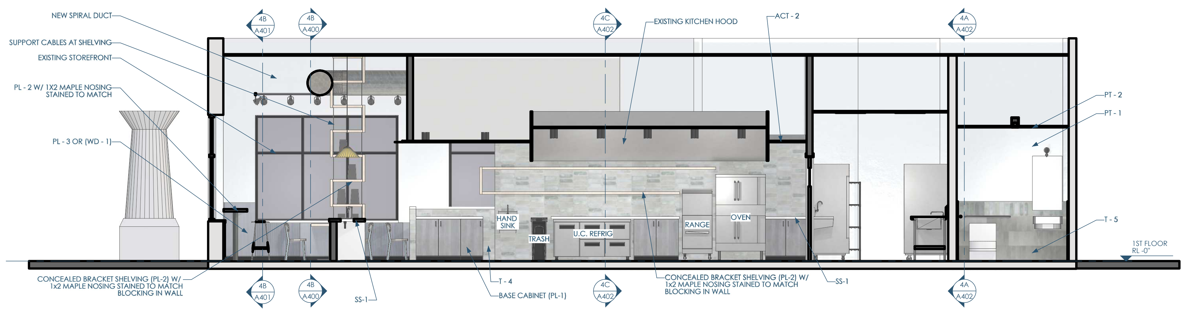
5B/A402 SECTION - N_S - EMP - E 1/4"=1'-0"
