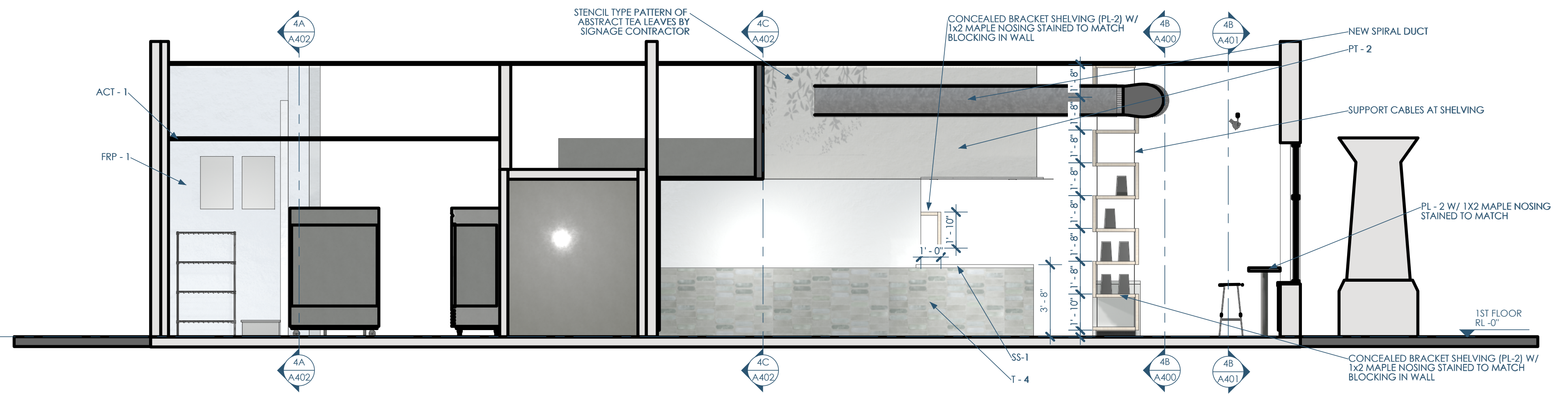
5A/A400 SECTION - N,S - DINING - W 1/4"=1'-0"
