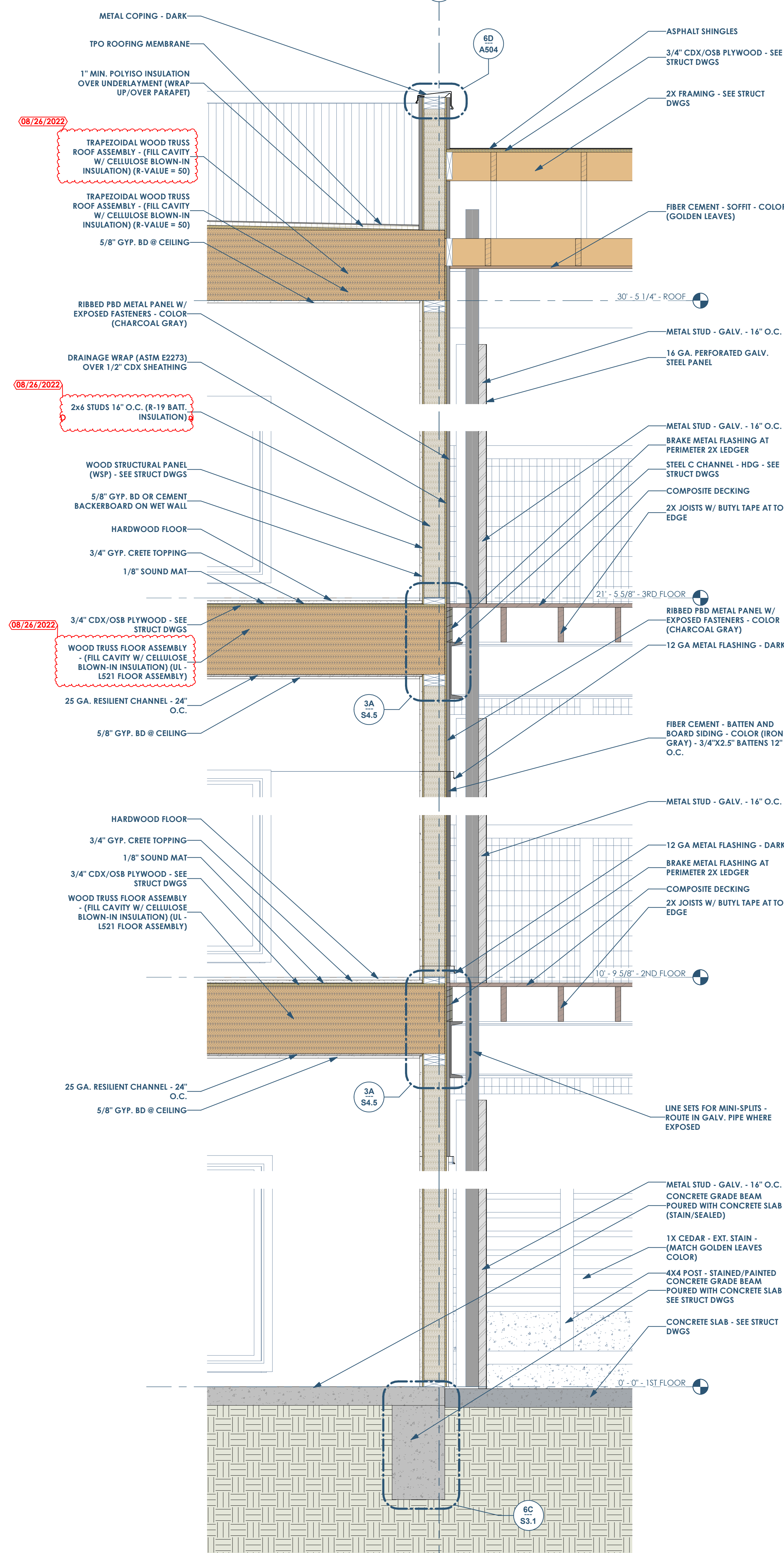
6A A402 BUILDING SECTION - EAST/WEST - AT SOUTH BALCONIES - LOOKING SOUTH (INT - EXT) 3/4" = 1'-0"
