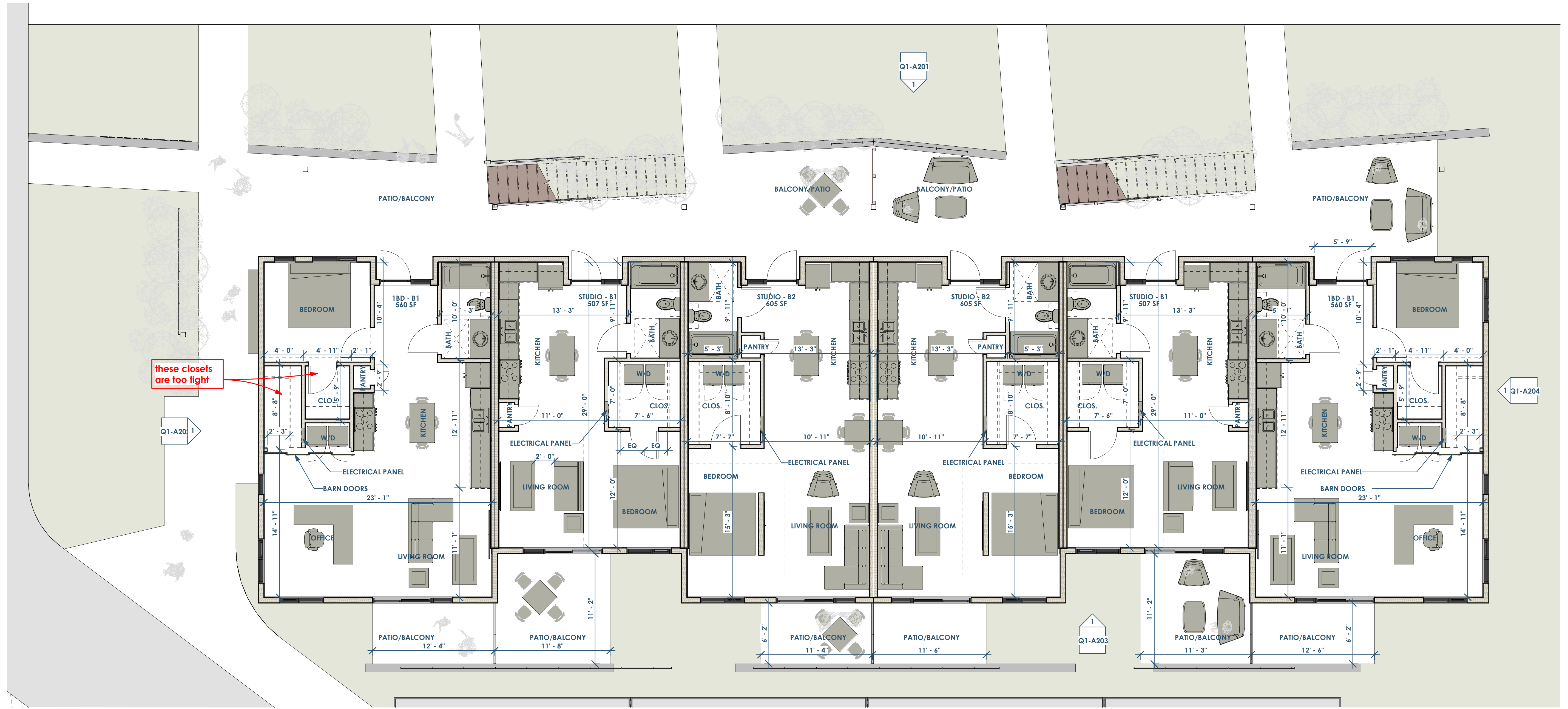
1 OPTION 2 - FLOOR PLAN - 1ST Q2-A101 3/16" = 1'-0"
