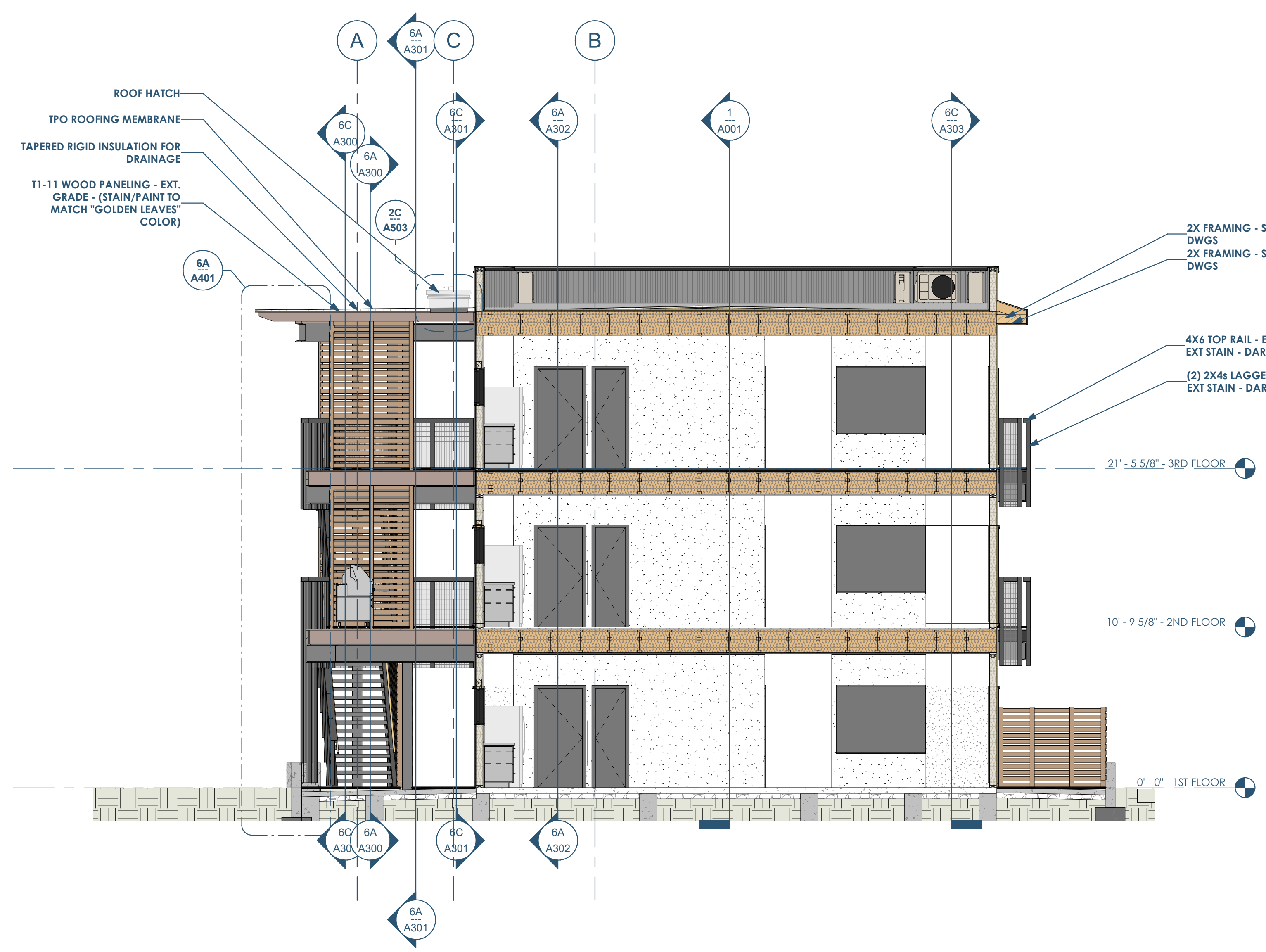
4C A302 BUILDING SECTION - THRU LARGE STUDIO - LOOKING EAST 3/16" = 1'-0"
