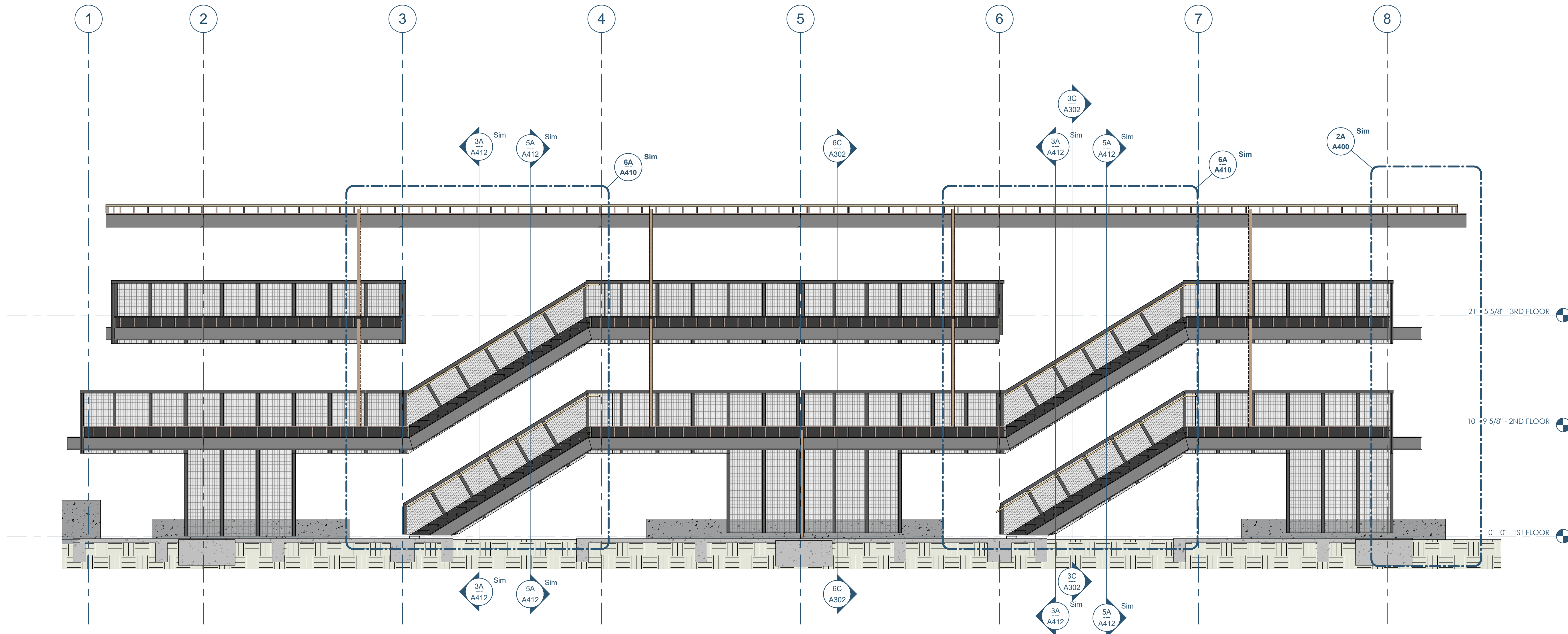
6C A300 BUILDING SECTION - THROUGH STAIRS - LOOKING NORTH 3/16" = 1'-0"
