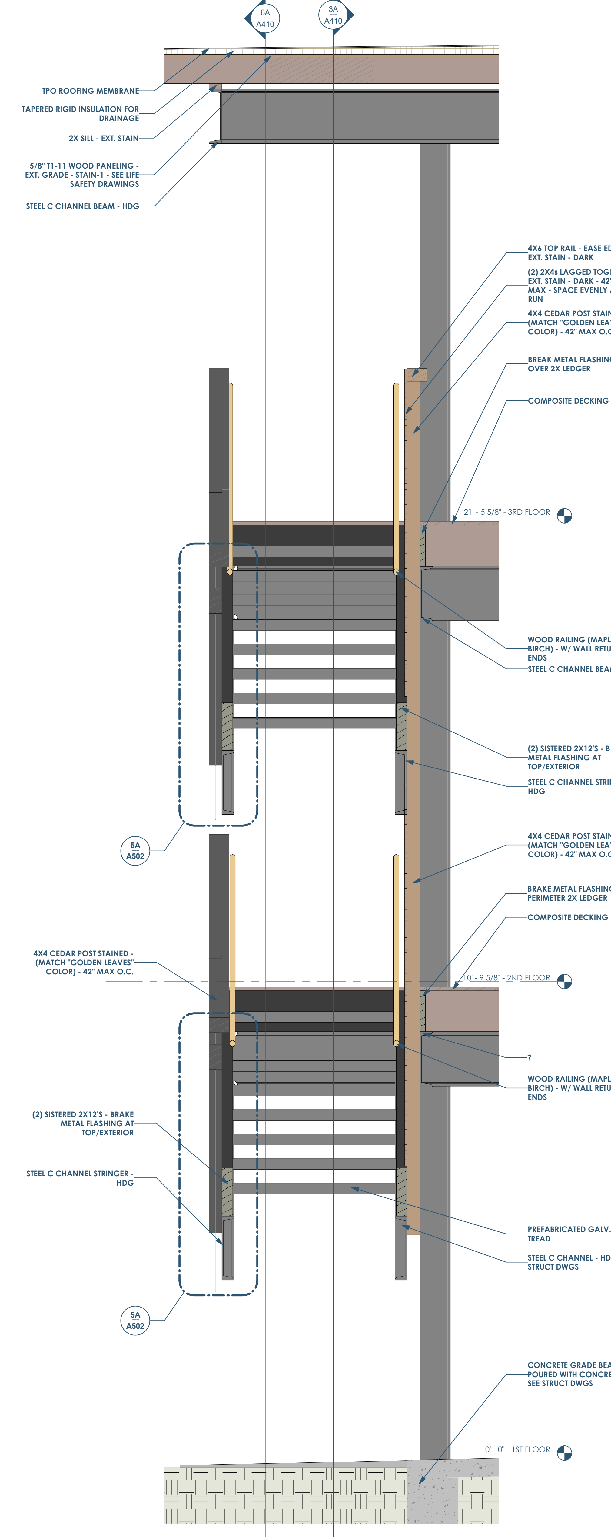
SA A412 STAIR SECTION - LOOKING EAST 3/4" = 1'-0"
