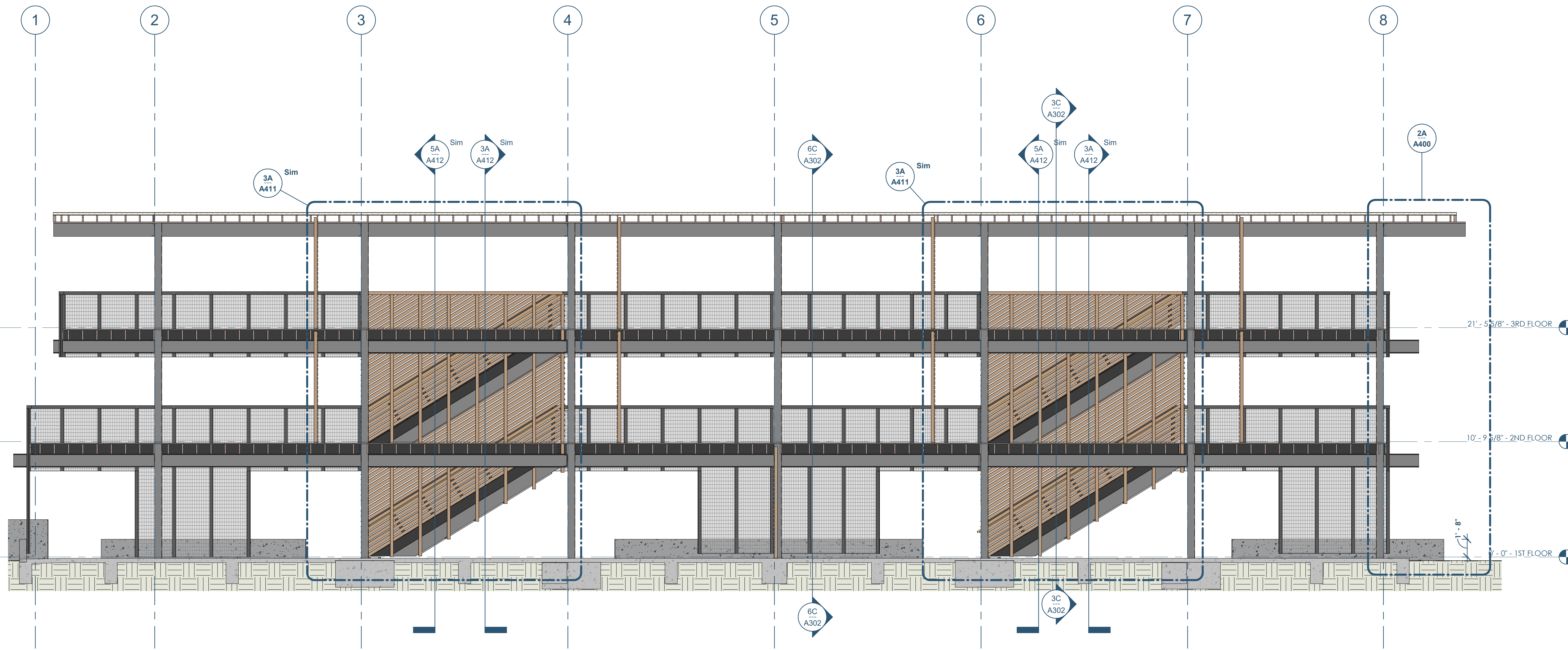
6C A301 BUILDING SECTION - THRU BALCONY - LOOKING SOUTH 3/16" = 1'-0"
