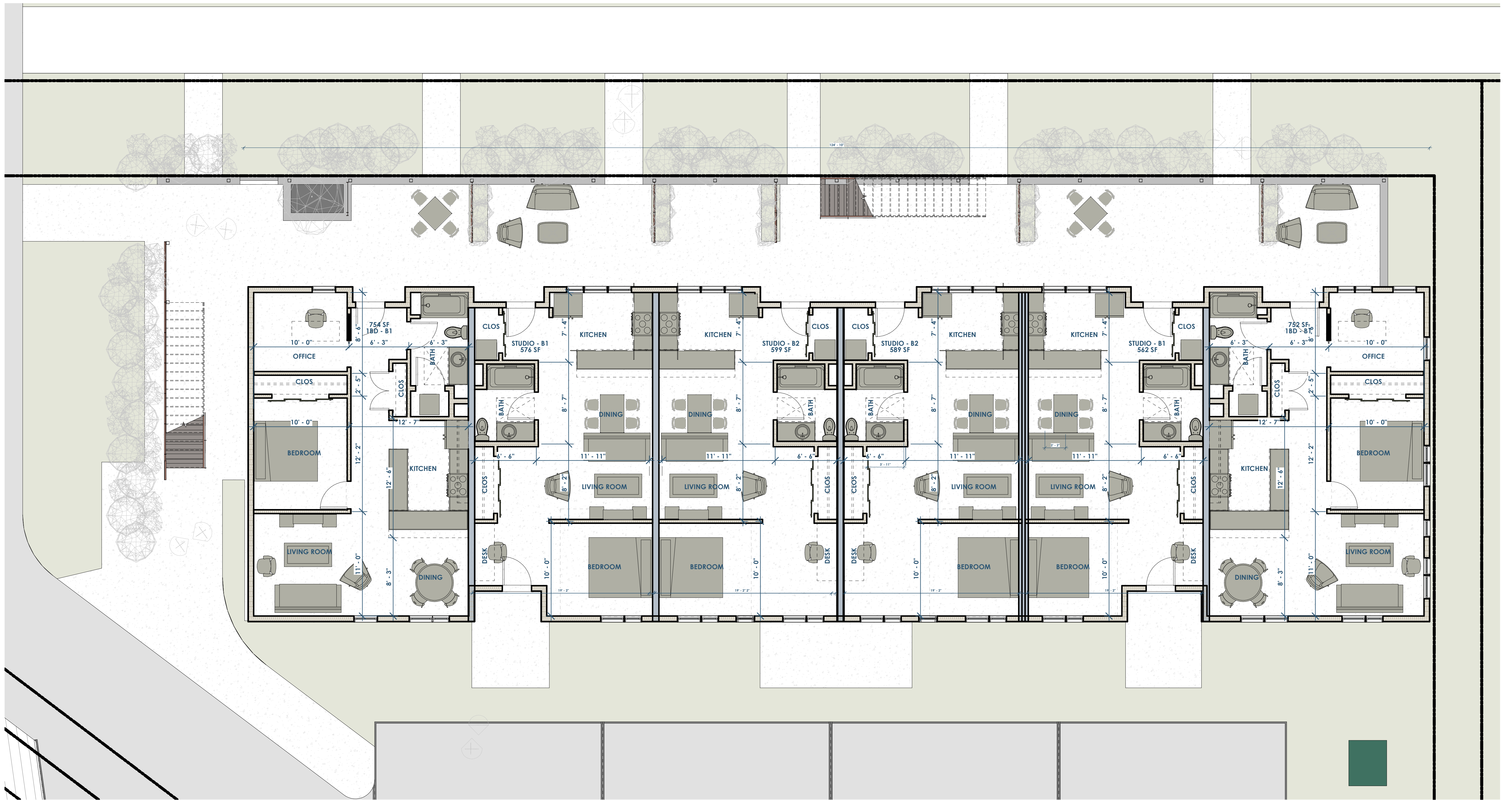
1 OPTION 3 - FLOOR PLAN - 1ST Q3-A101 3/16" = 1'-0"
